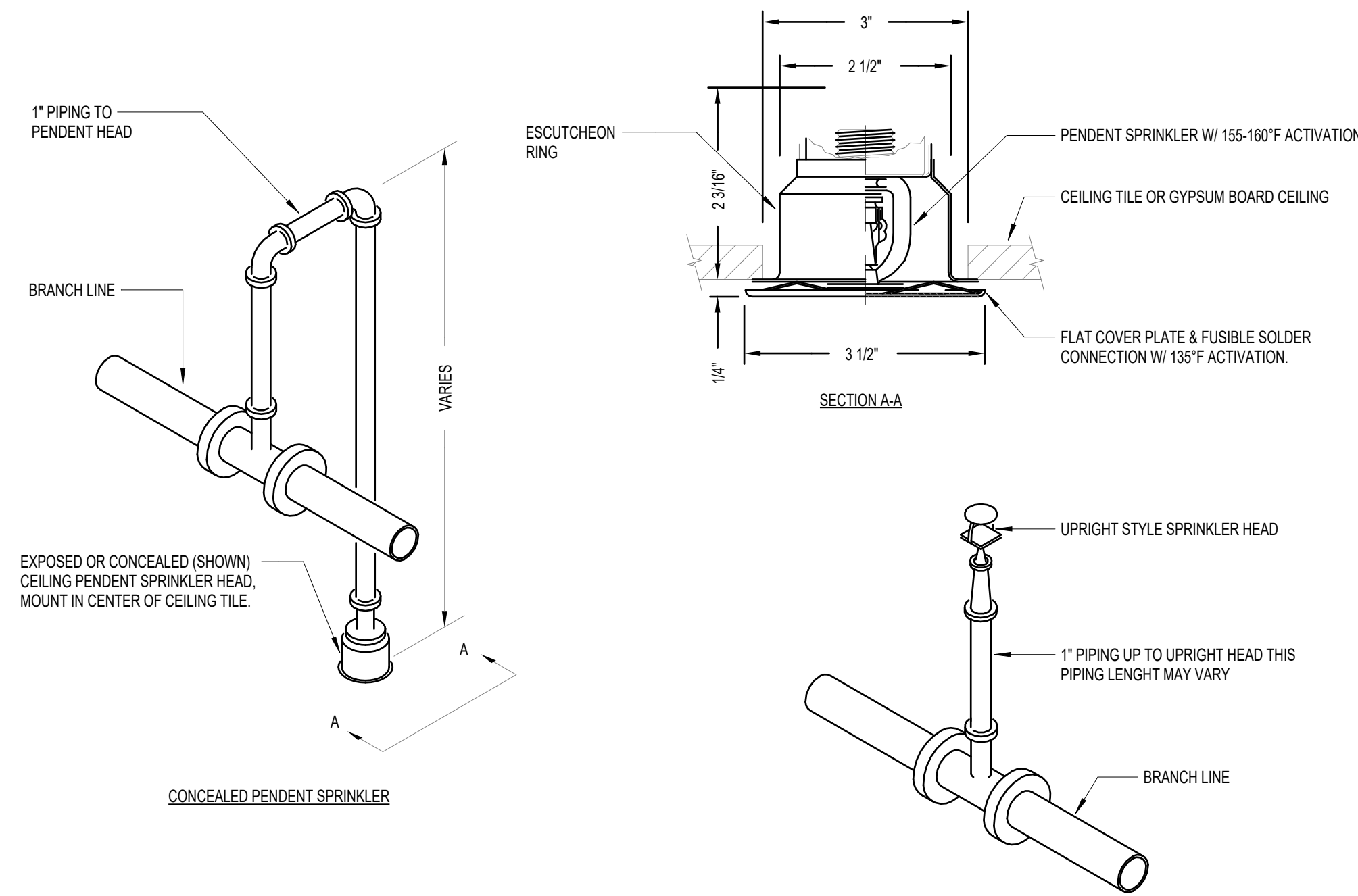
E2 CONCEALED SPRINKLER ARM OVER AND UPRIGHT SPRINKLER NOT TO SCALE
