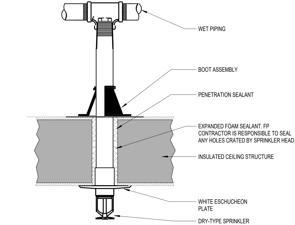
E5 DRY-TYPE SPRINKLER INSTALLATION NOT TO SCALE
