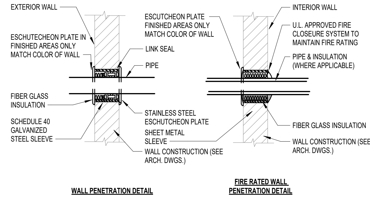
E3 WALL PENETRATION NOT TO SCALE
