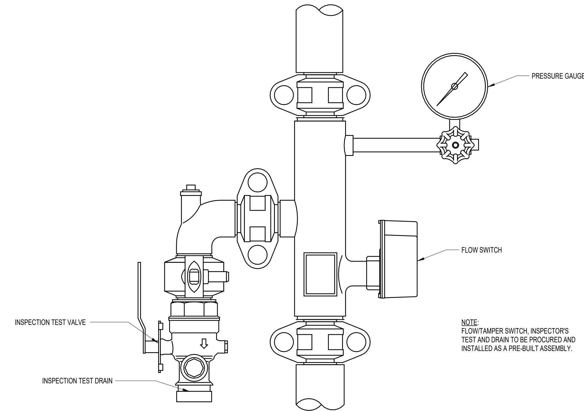
C2 INSPECTORS TEST AND FLOW SWITCH ASSEMBLY NOT TO SCALE
