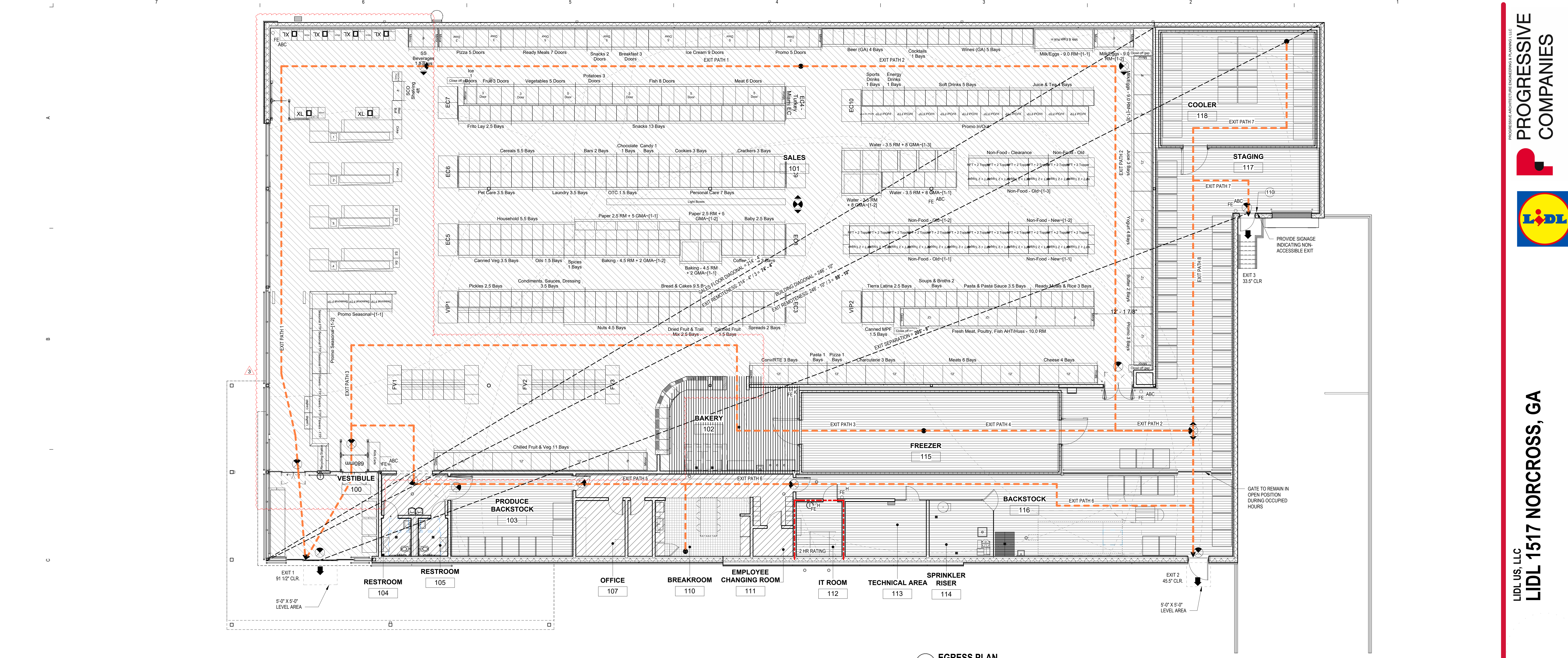
EGRESS PLAN 1/8" = 1'-0"
