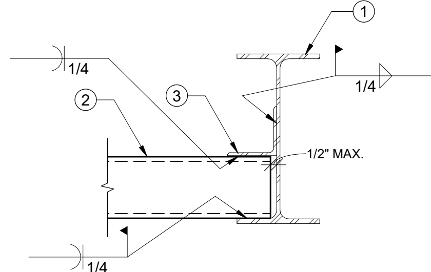
8 HSS TO W-BEAM CONNECTION 1 1/2" = 1'-0"
