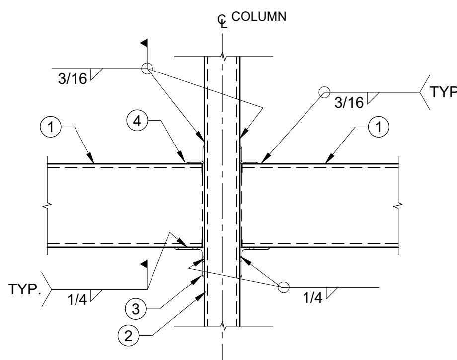
10 TOP OF VESTIBULE POST BRACING 1" = 1'-0"
