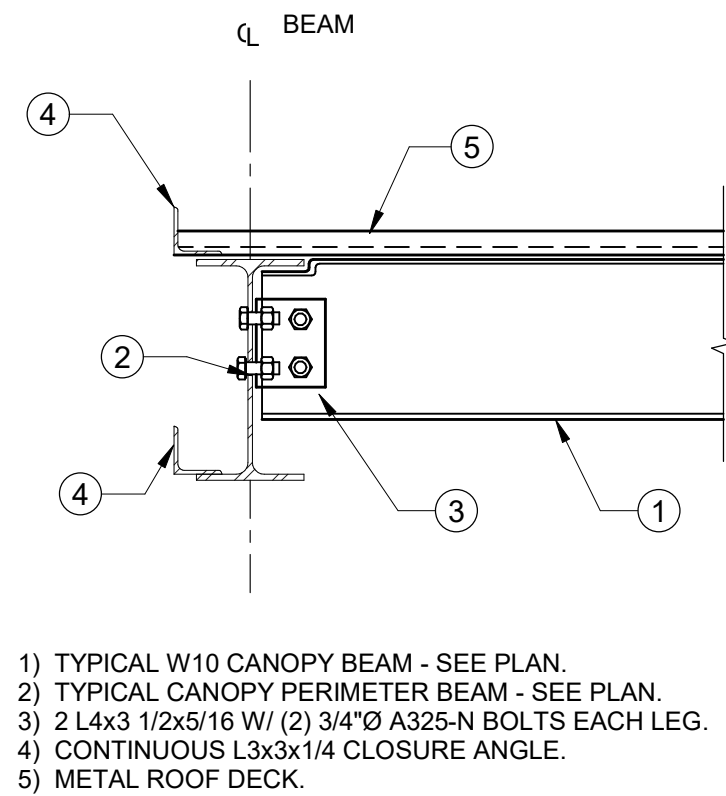
4 TYPICAL CANOPY BEAM AND EDGE DETAIL 1" = 1'-0"
