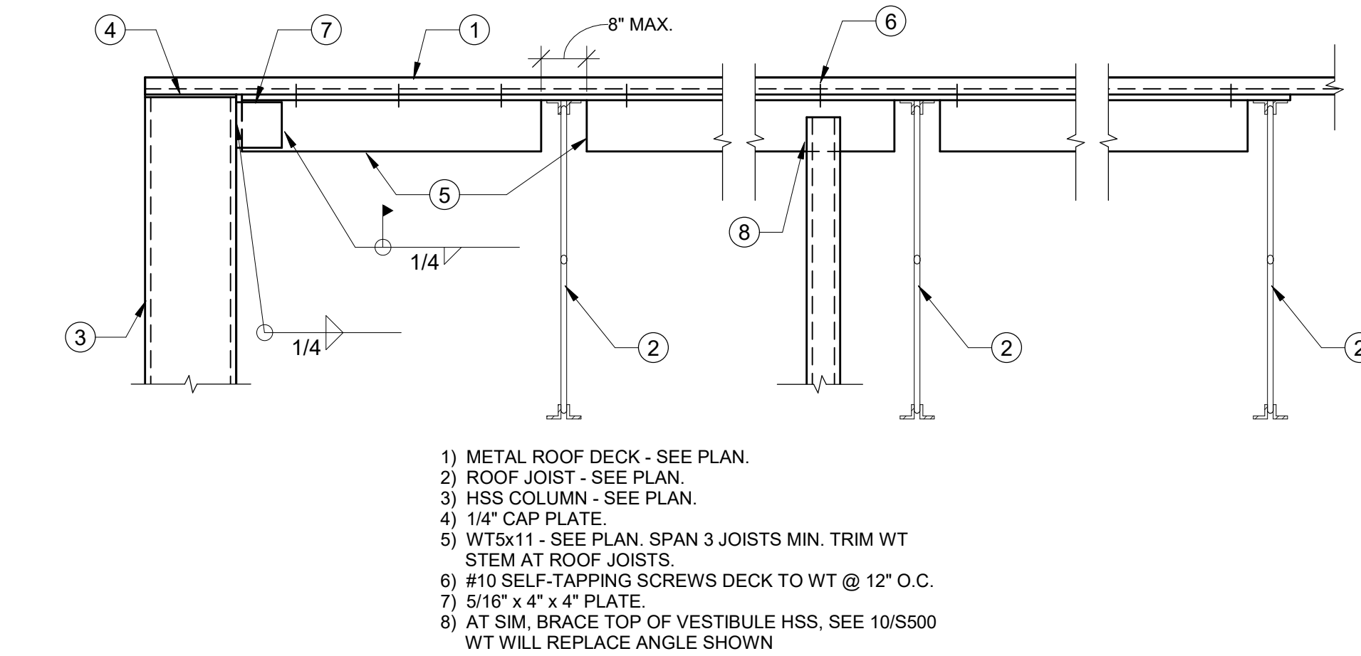
9 WT BRACE AT HSS POST 1" = 1'-0"
