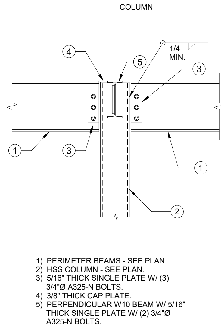
5 TYPICAL WIDE FLANGE BEAM TO COLUMN DETAIL 3/4" = 1'-0"
