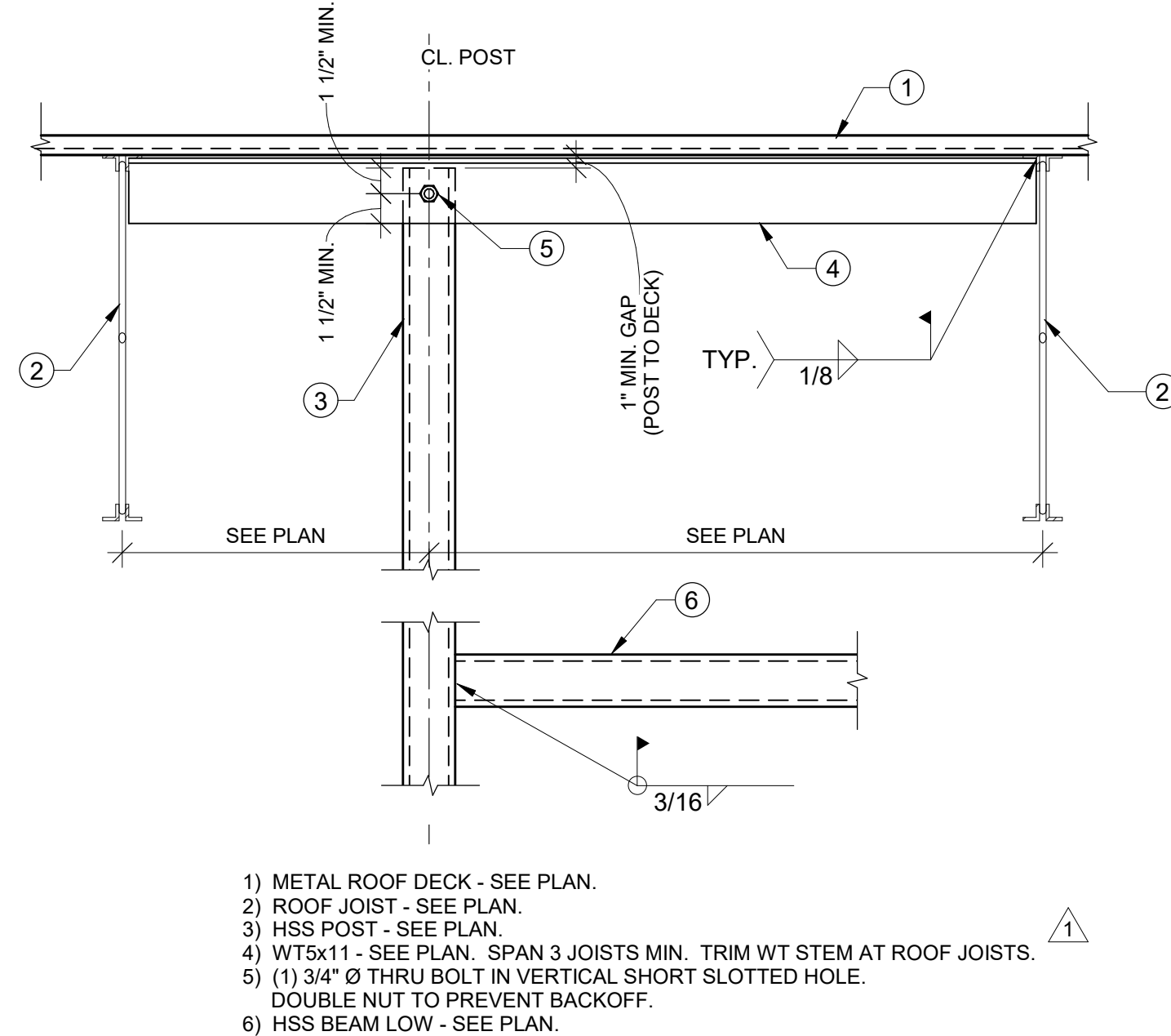
10 TOP OF VESTIBULE POST BRACING 1" = 1'-0"
