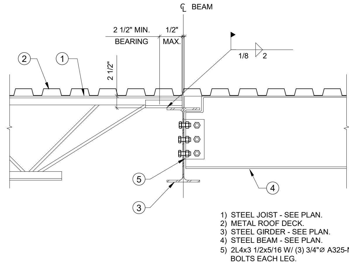
7 "K" JOIST AND STEEL BEAM BEARING ON STEEL GIRDER N.T.S.
