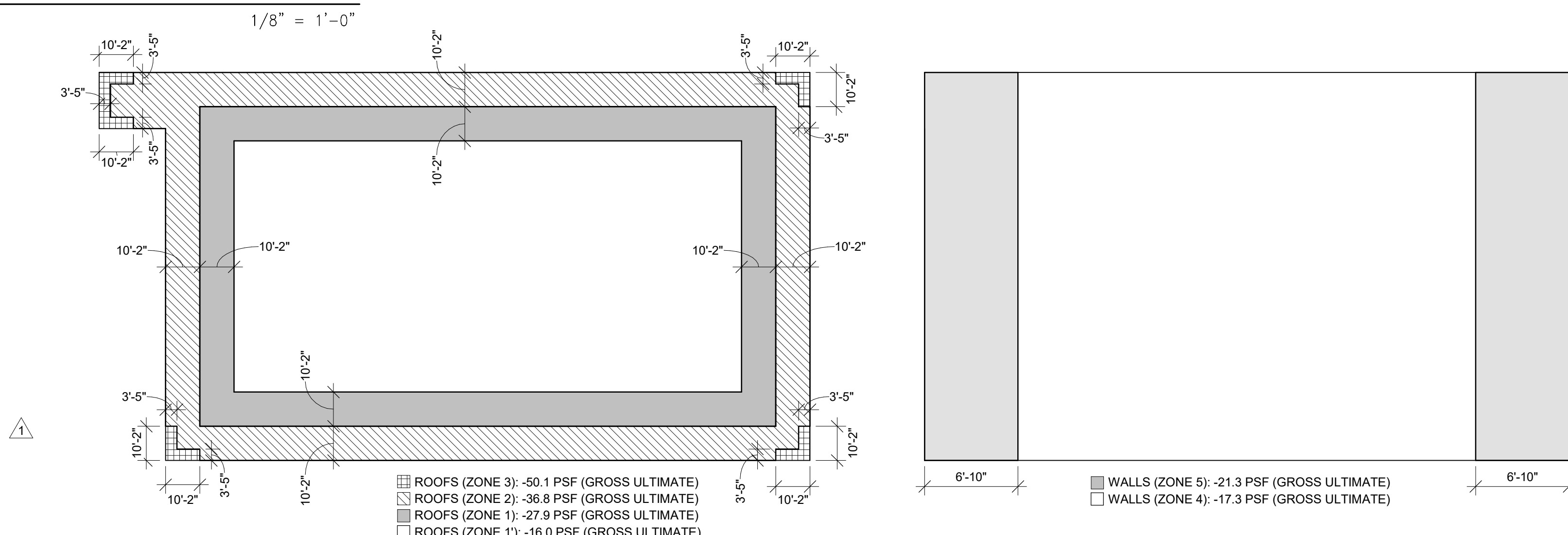
WIND UPLIFT DIAGRAM AND C&C WALL LOADS
