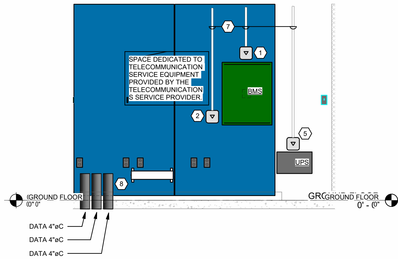
2 TECHNICAL ROOM - PLAN EAST WALL ELEVATION
