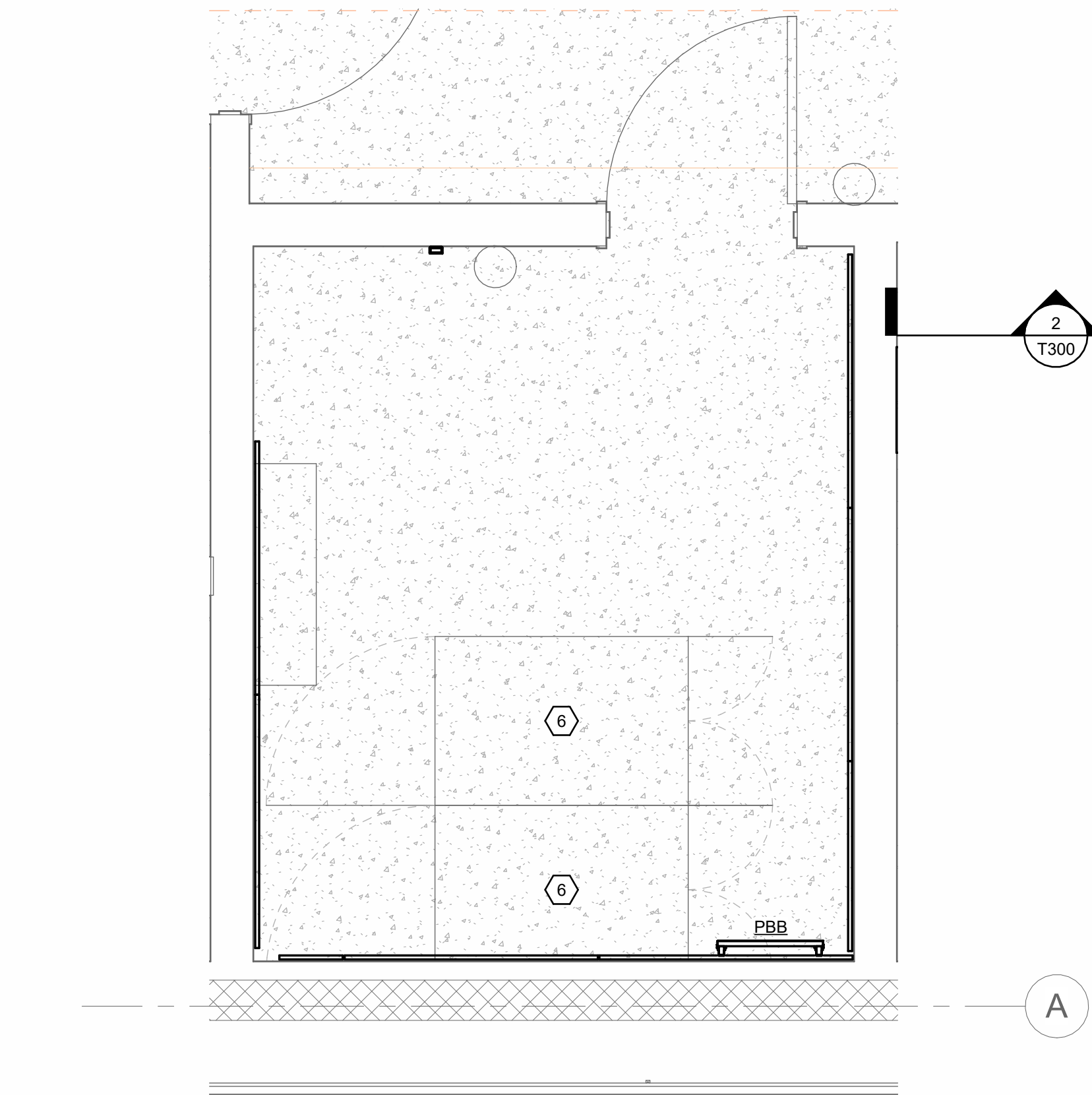
3 IT ROOM - ENLARGED TECHNOLOGY PLAN
