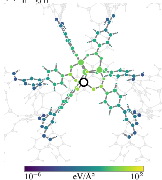
(c) \|\Phi_{ij}\| from that atom
