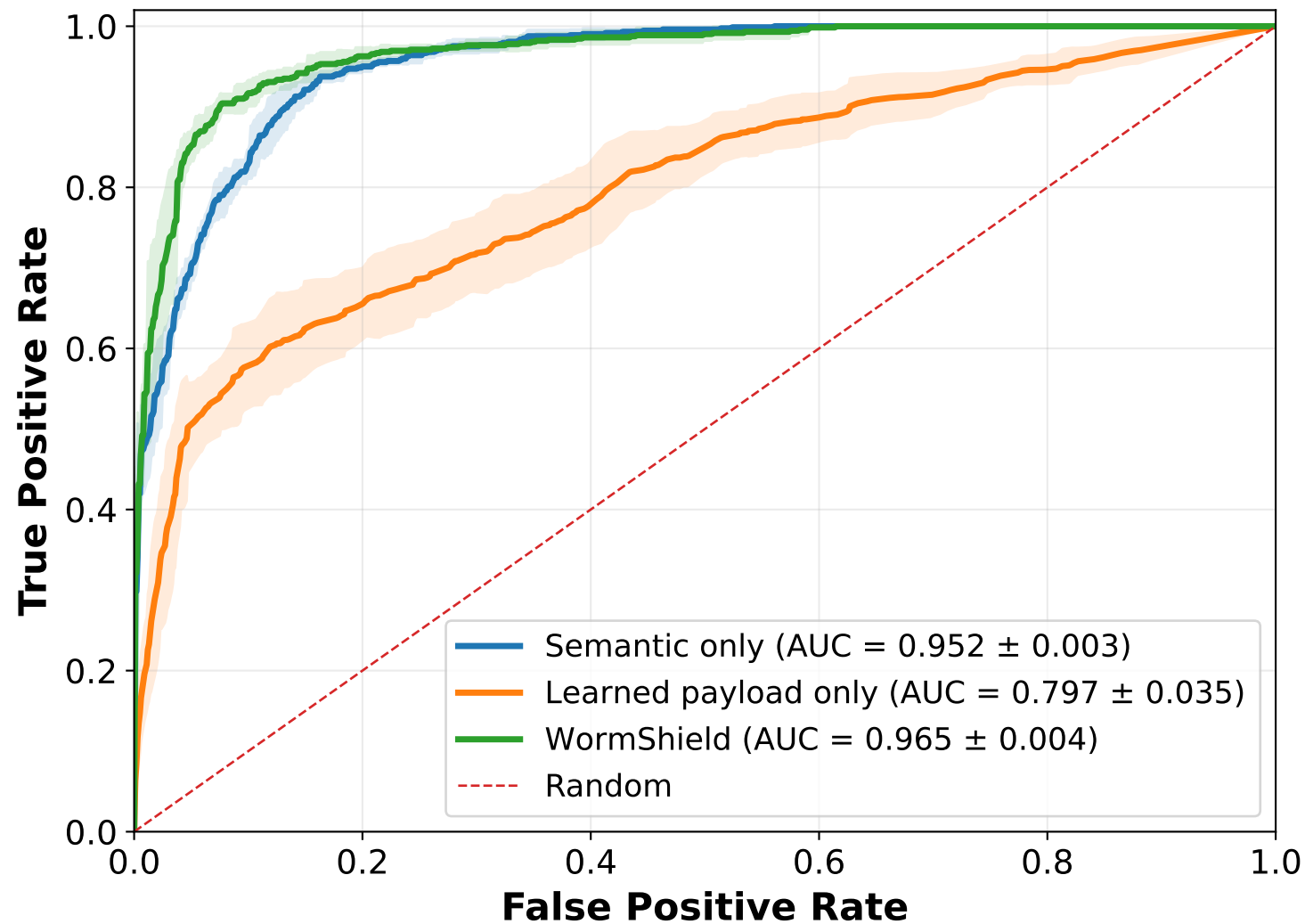
ROC Curves on AgentArena
