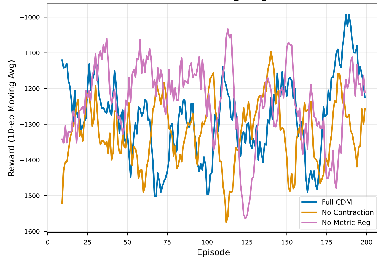
Learning Reliability
