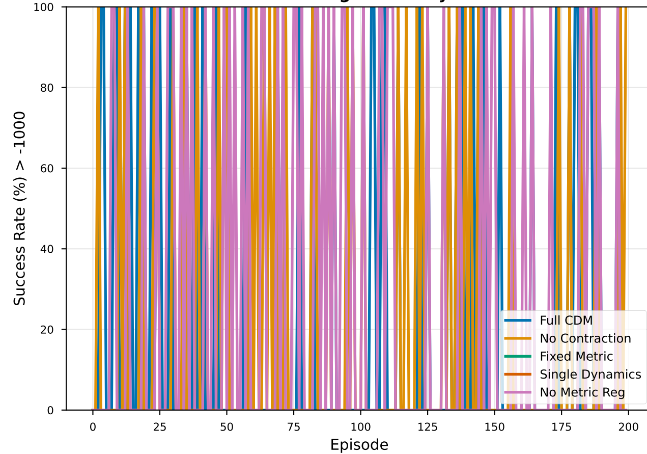
Learning Reliability
