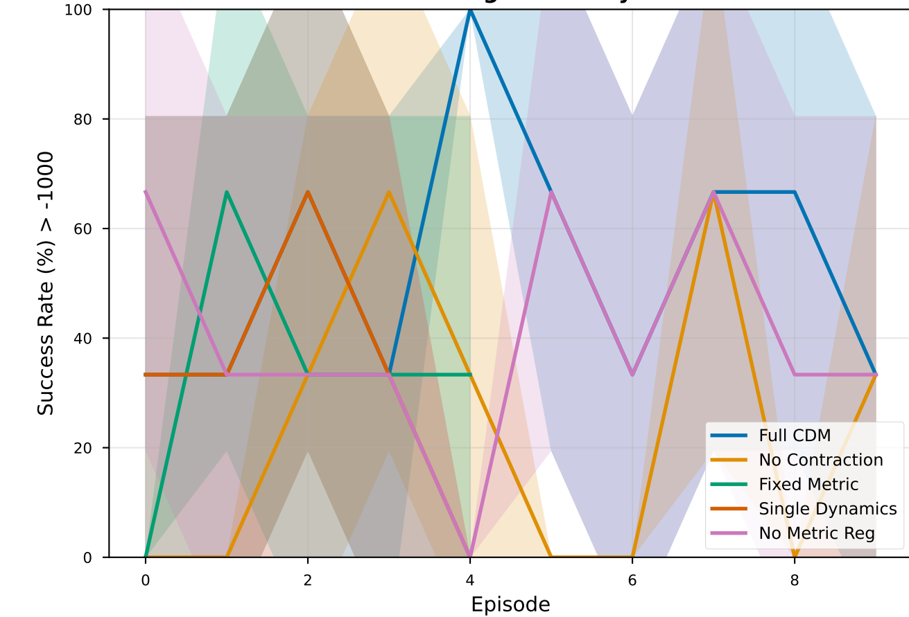
Learning Reliability
