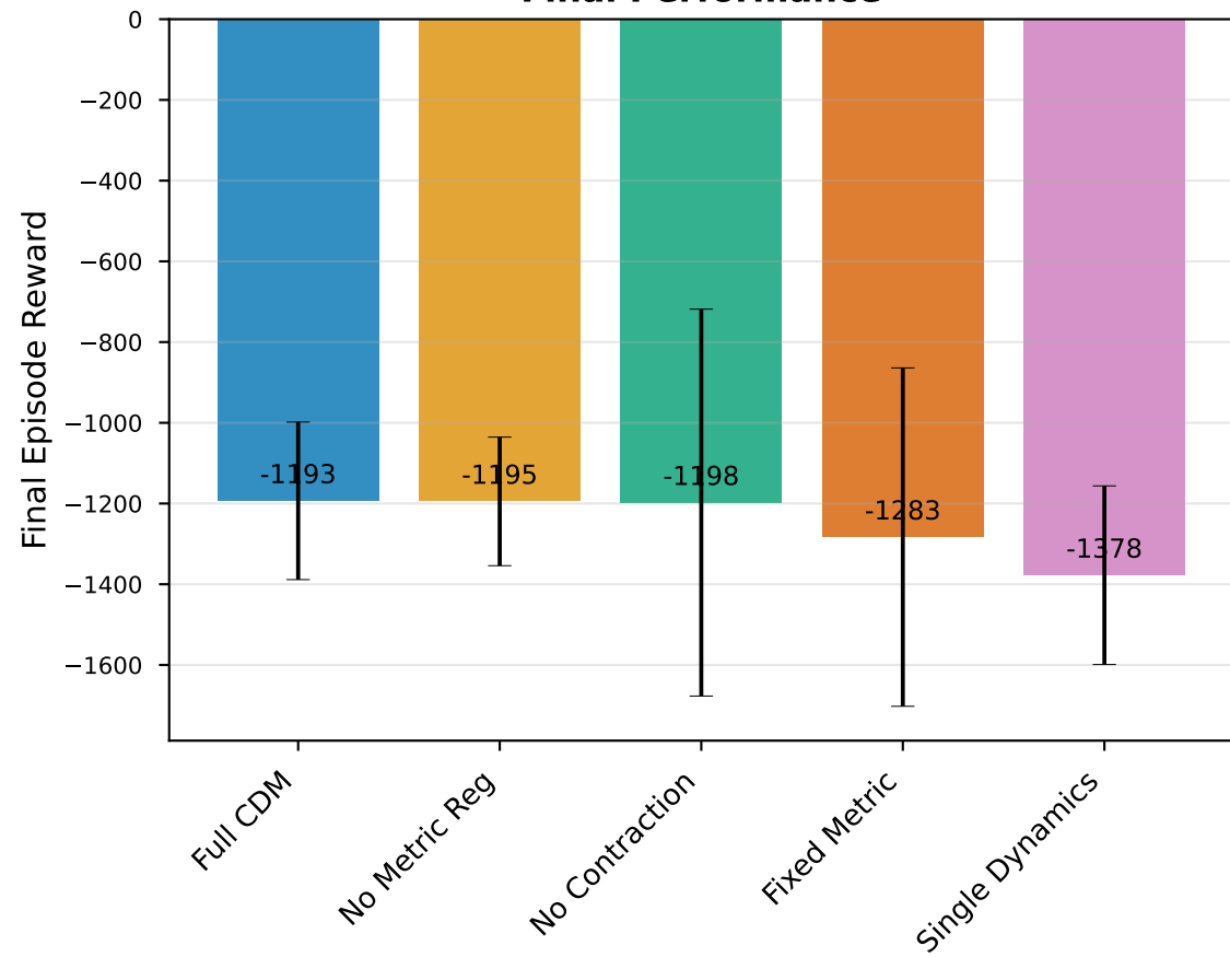
Final Performance
