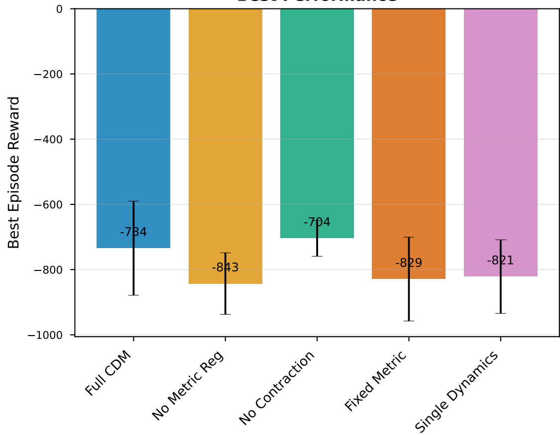
Best Performance
