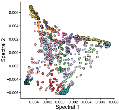
Embeddings of 22 clusters
