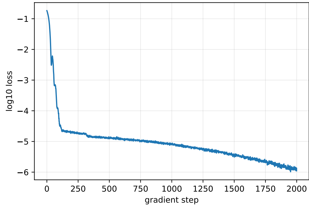
Training loss
