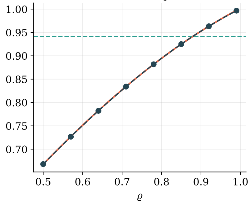
Autocorr(log Y)
