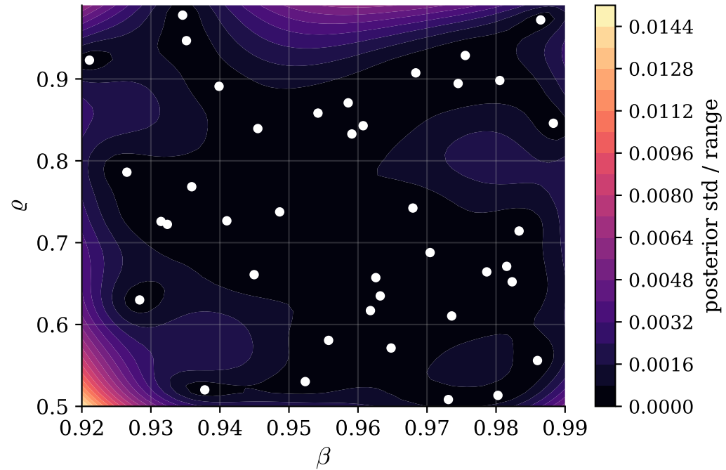
where the GP is unsure
