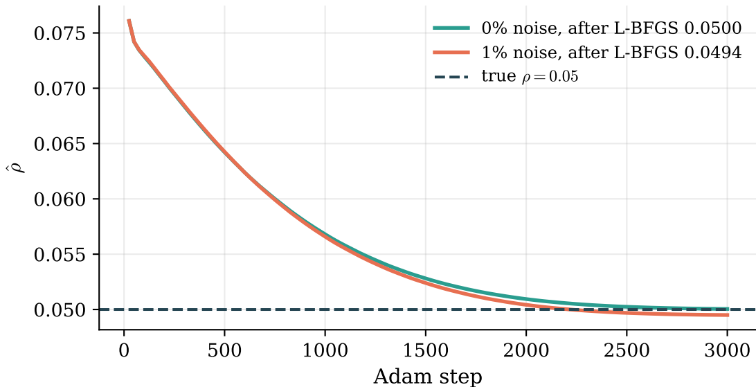
recovering \rho from 20 consumption observations
