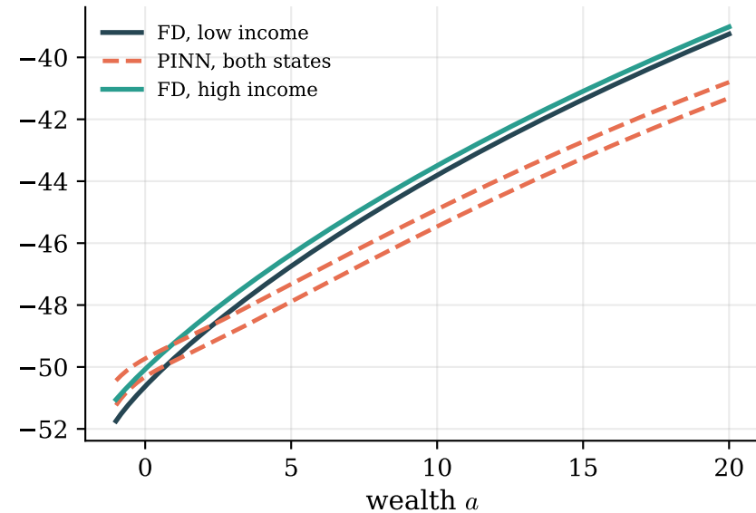
value functions
