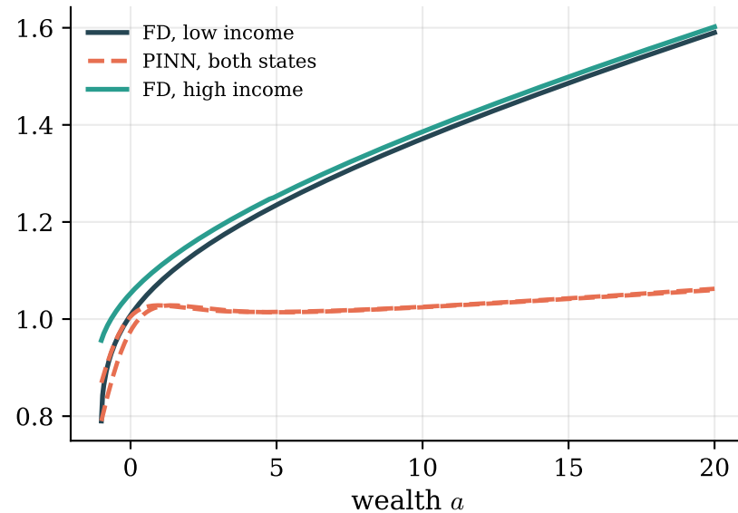
consumption policies
