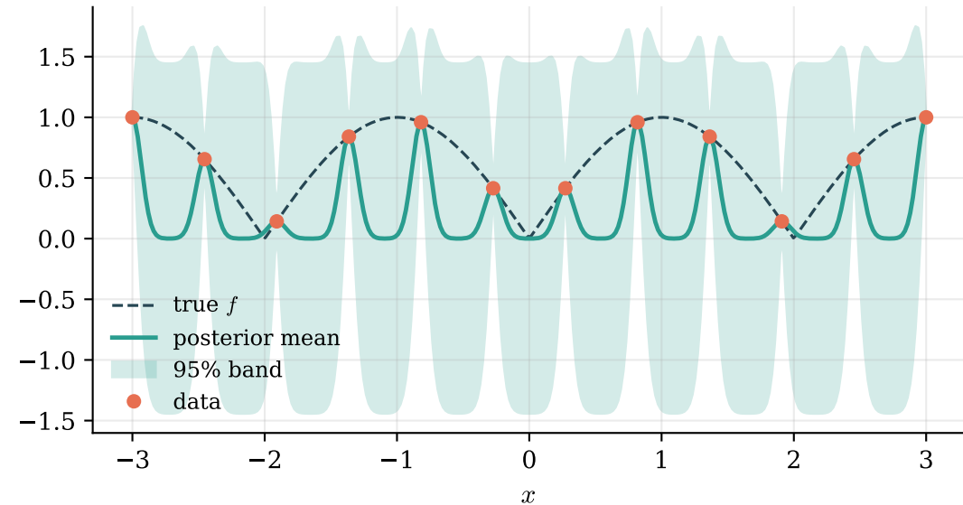
squared exponential, log ML -13.3
