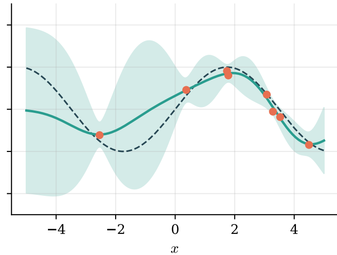
noisy labels, \sigma_y = 0.15
