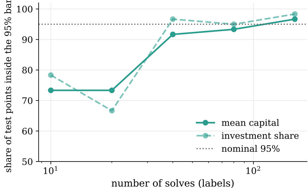
calibration of the GP's error bar
