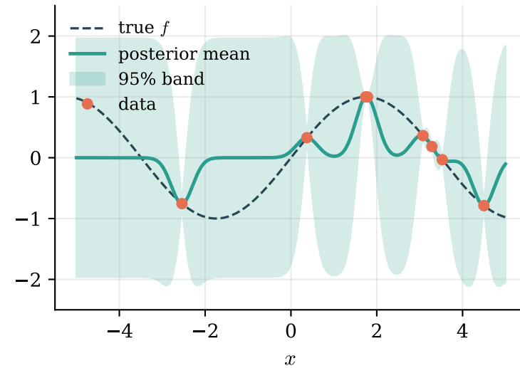
\ell = 0.25
