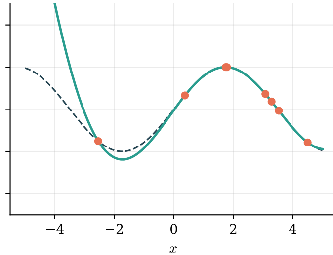
\ell = 5.0
