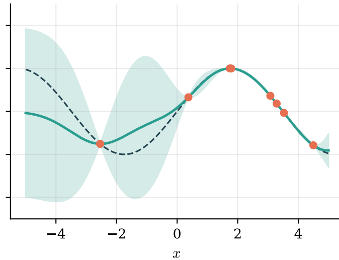
\ell = 1.0
