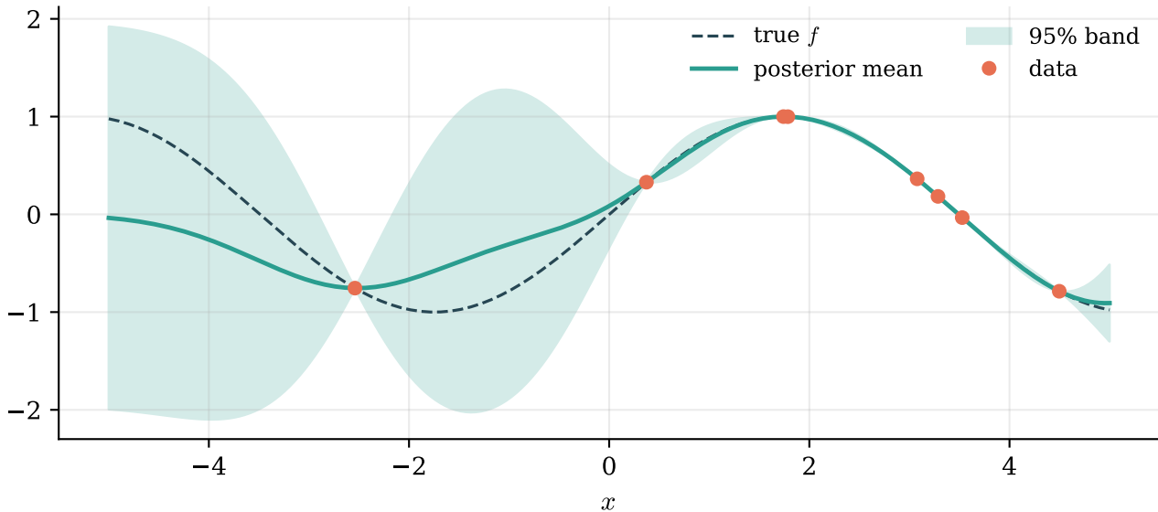
GP posterior from scratch, 8 points
