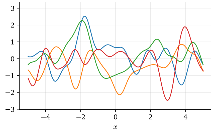
prior samples, \ell = 0.5
