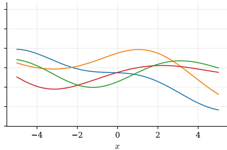
prior samples, \ell = 3.0
