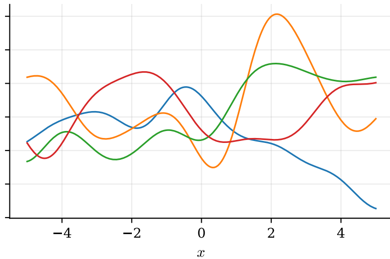
prior samples, \ell = 1.0
