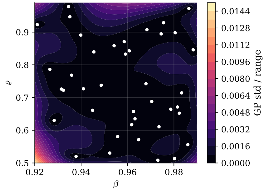
where the GP is unsure
