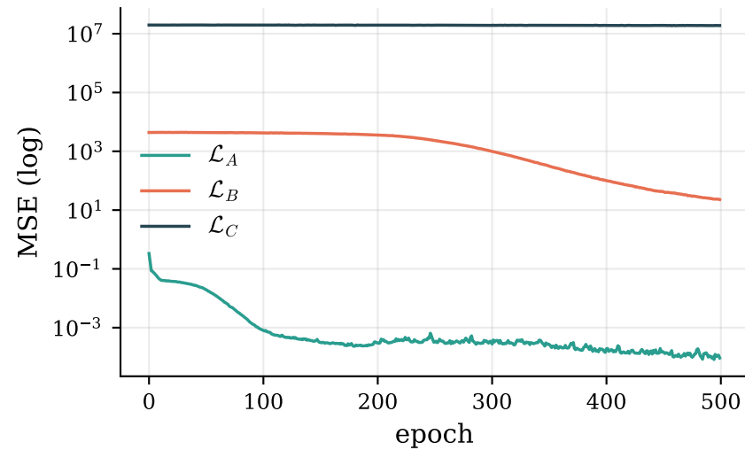
Component losses
