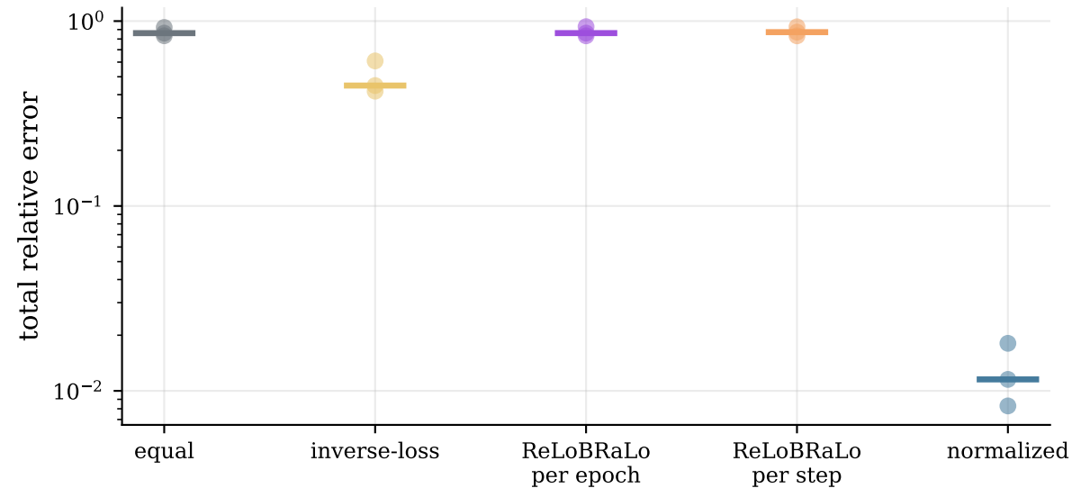
Every seed, with the median marked
