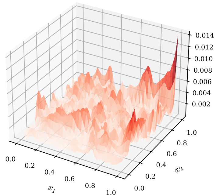
|f - \hat{f}|
