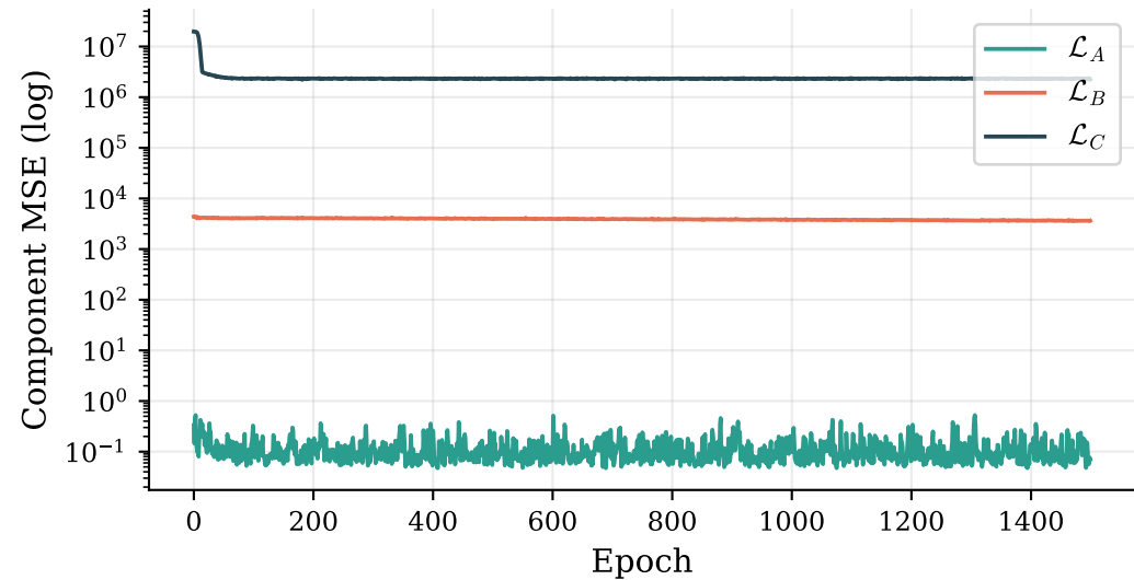
Component losses
