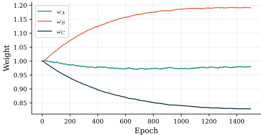
Component weights
