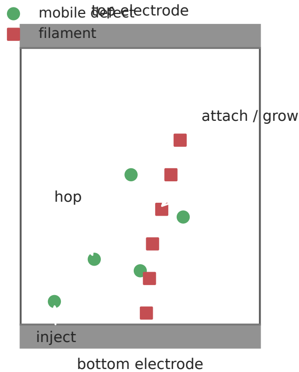
(b) Lattice KMC states and events
