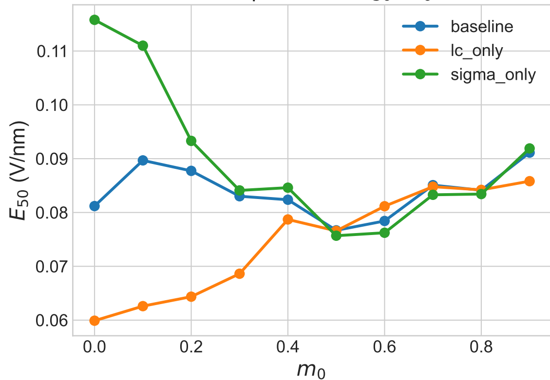
Decomposition of E_{50}(m_0)
