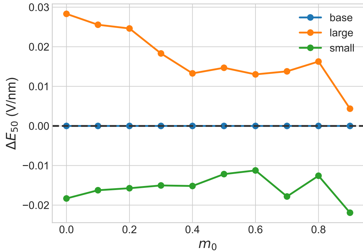
Lattice-size robustness of threshold field
