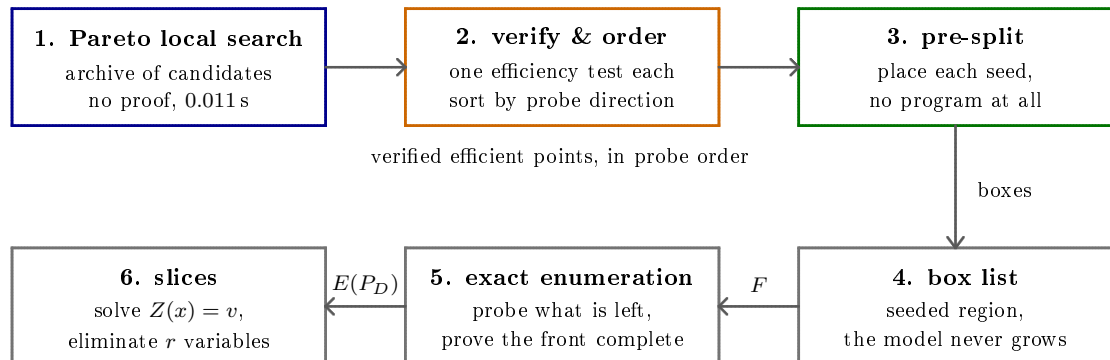
Figure 1: Process structure. Only verified efficient points cross from the heuristic side to the exact side, and they cross in probe order. Nothing crosses back: the heuristic never sees the exact phase’s findings, which is why its cost is a one-off.
