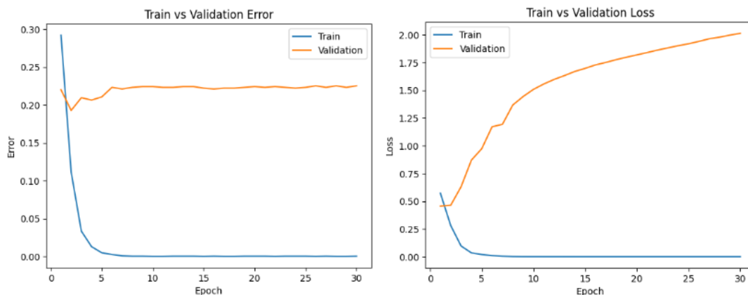
Figure 6: Train vs Validation Error and Loss showing overfitting after Epoch 3.
