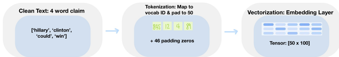
Figure 4: Pipeline of raw text tokenization, padding, and embedding vectorization.
