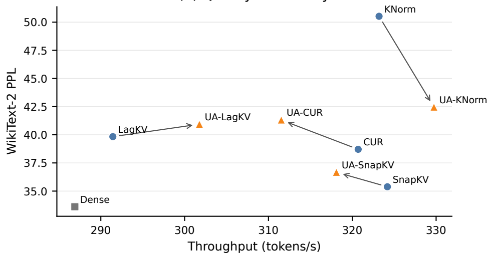
(b) Quality--Efficiency
