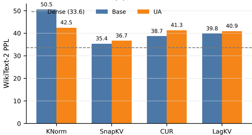
(a) Main PPL
