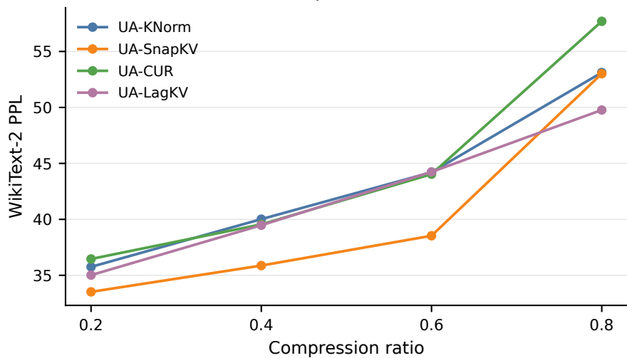
(c) Compression Ratio
