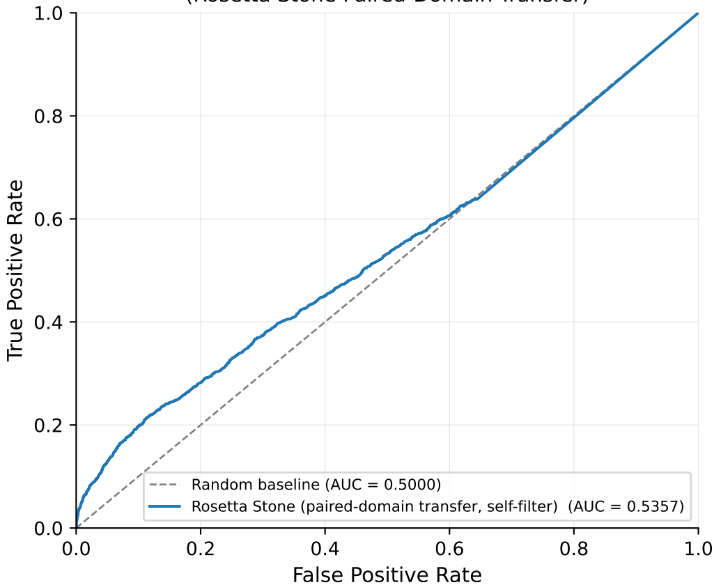
ROC Curve (Rosetta Stone Paired-Domain Transfer)
