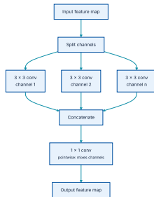
Figure 9.4 — a depthwise convolution (independent spatial convolutions per channel) followed by a pointwise 1 \times 1 convolution that mixes channels.
