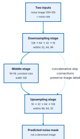
Figure 17.9 — a 1:1 mapping between downsampling and upsampling blocks.
