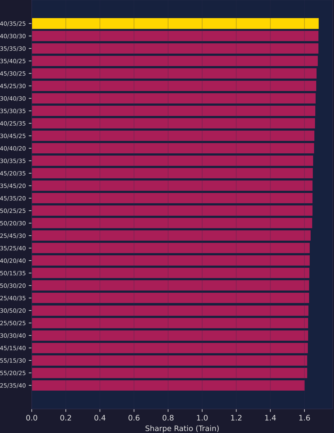
Top 30 Weight Combos by Sharpe
