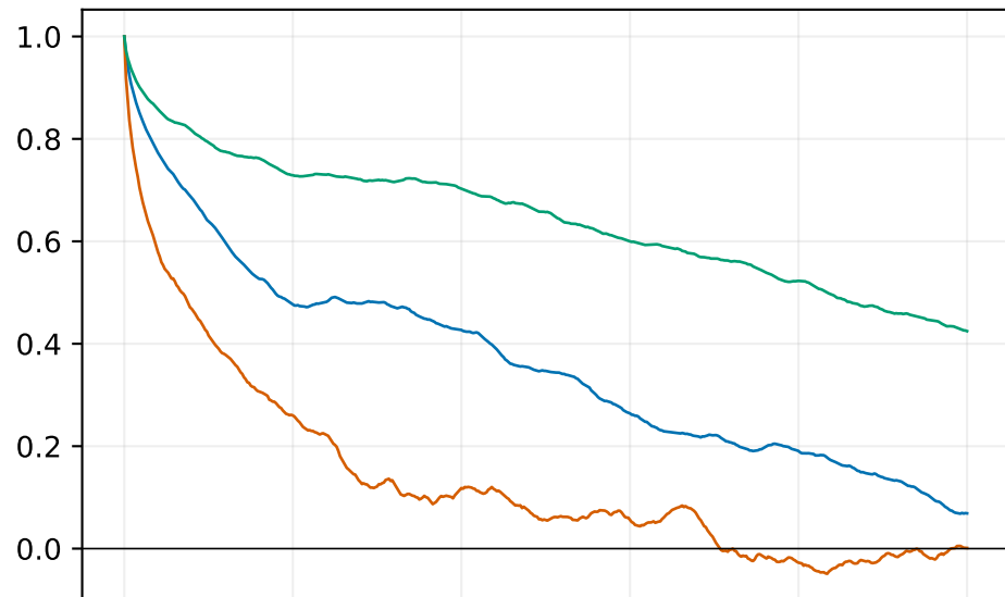
End-to-end distance (A)
