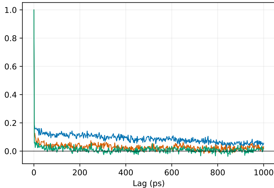
PFOA-polymer minimum (A)
