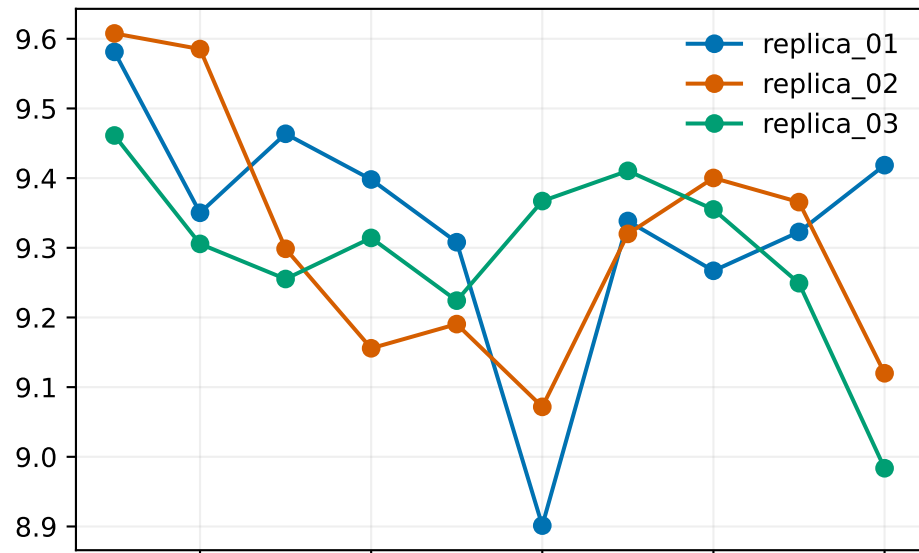
Polymer Rg (A)
