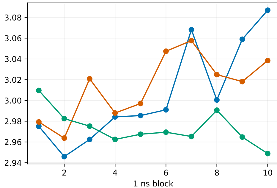
PFOA-polymer minimum (A)
