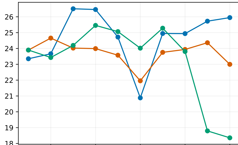
End-to-end distance (A)
