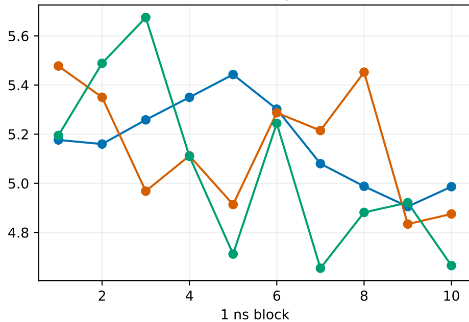
PFOA head-any N (A)
