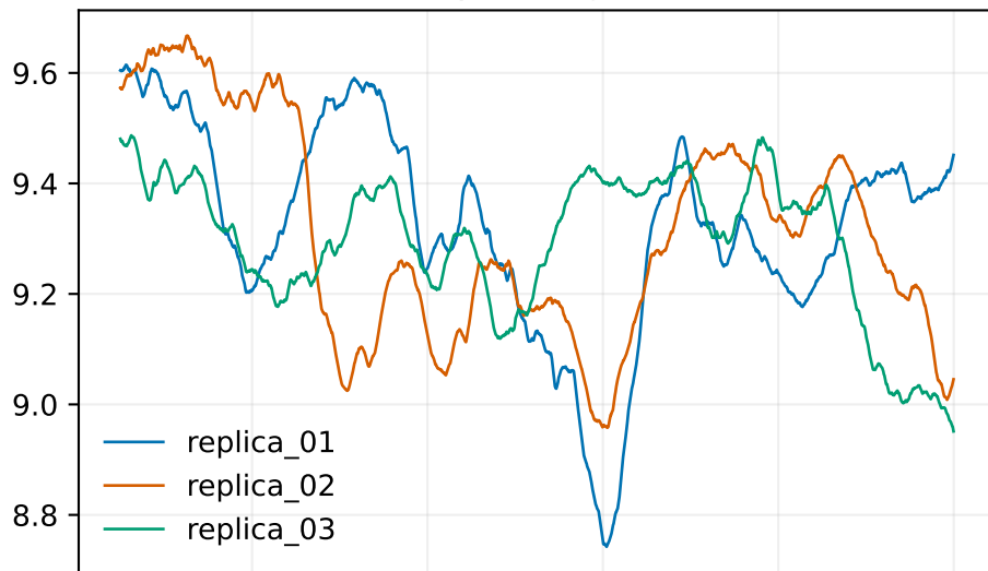
Polymer Rg (A)
