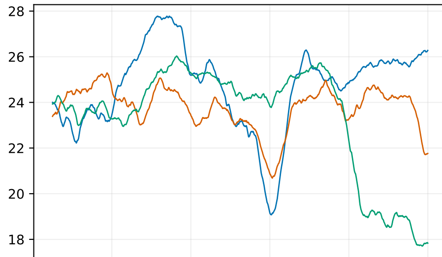
End-to-end distance (A)
