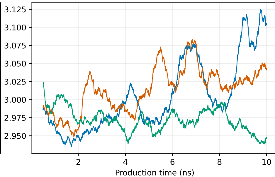
PFOA-polymer minimum (A)
