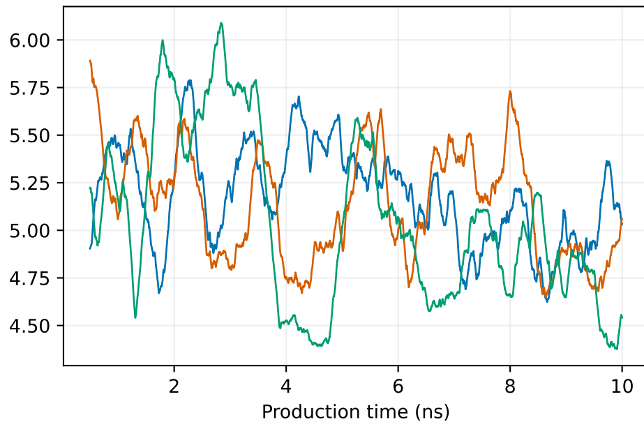
PFOA head-any N (A)
