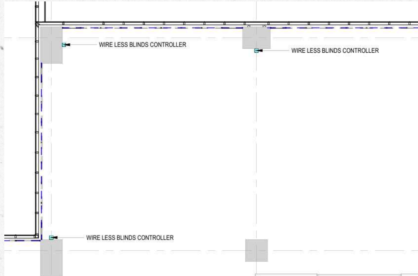
BLIND-PLAN VIEW
