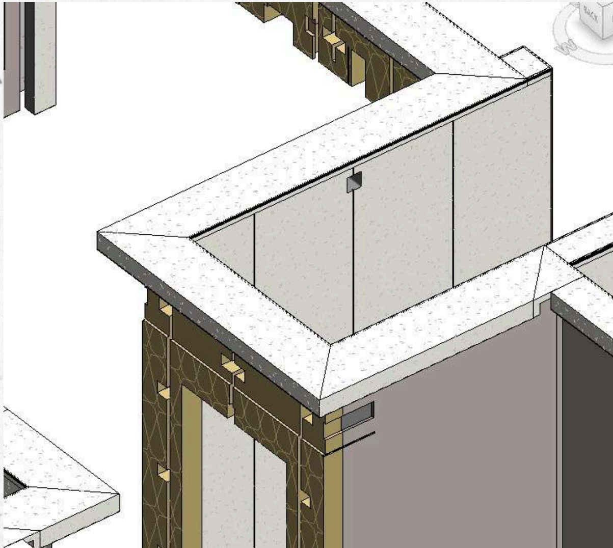
ISOMETRIC VIEW- COPING
