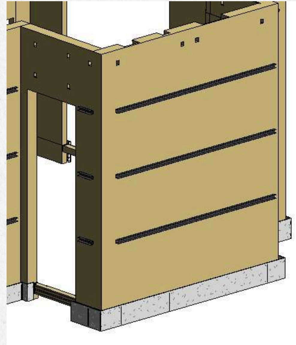
SKIRTING VIEW- CEMENT BOARD
