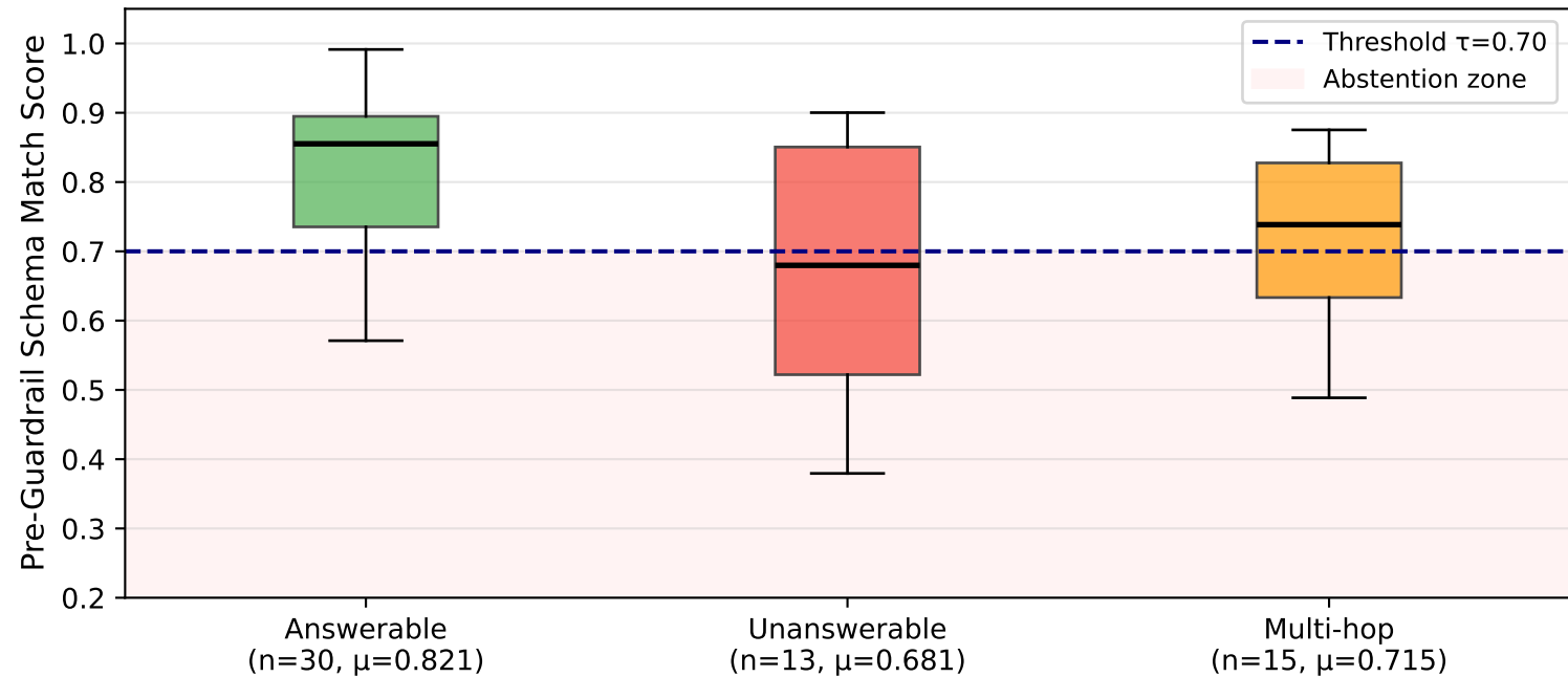
Pre-Generation Guardrail Score Distribution by Query Type ( t=3.072 , p=0.0038^{**} , Cohen's d=0.942 )
