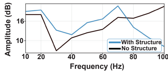
Fig. 25. The amplification effect of the C-shaped frame.
