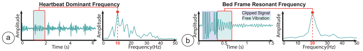
Fig. 9. (a) The dominant frequency of heartbeat-induced vibration is around 10Hz, and (b) the peak resonant frequency of the bed frame is around 20Hz.
