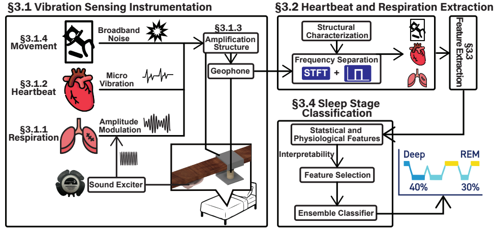
Fig. 2. System Overview of SleepVibe
