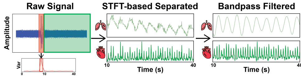
Fig. 4. SleepVibe signal processing pipeline.
