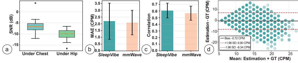
Fig. 18. Respiratory effort evaluation across real sleep sessions. (a) The geophone under the chest provides the higher respiratory SNR on average. (b)&(c) SleepVibe achieves respiratory rate accuracy and waveform-level correlation comparable to mmWave sensing. (d) Bland-Altman analysis of SleepVibe respiratory rate estimation.
