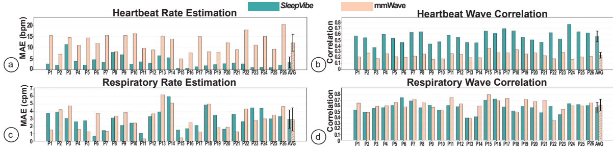
Fig. 19. Controlled physiological evaluation across 26 participants. Panels (a) and (b) show the heart rate MAE and waveform correlation, respectively. Panels (c) and (d) show the respiratory rate MAE and waveform correlation. SleepVibe significantly outperforms mmWave in heartbeat monitoring (two-sided t -test, p < 0.001 ) while achieving comparable respiratory monitoring performance.
