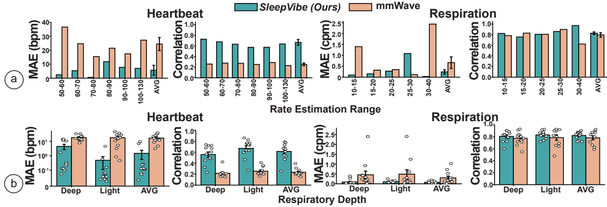
Fig. 21. Robustness to physiological variation. (a) Elevated heart and respiratory rates. (b) Deep and light breathing.
