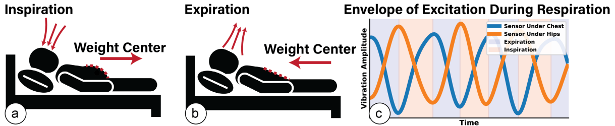
Fig. 3. The insight of the active vibration sensing for respiration. (a) During inspiration, the body weight center shifts toward the leg of the bed. (b) During expiration, the body weight shifts back. (c) This diaphragmatic breathing leads to a slow-cycle body weight shift that impacts the excitation signal amplitude following the respiration cycle.
