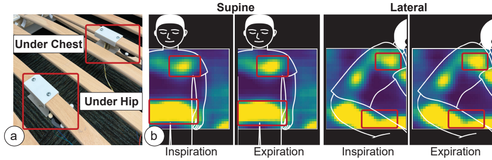
Fig. 8. (a) The optimal geophone placement under the chest and hip regions is guided by (b) the characterization of pressure distribution during respiration.
