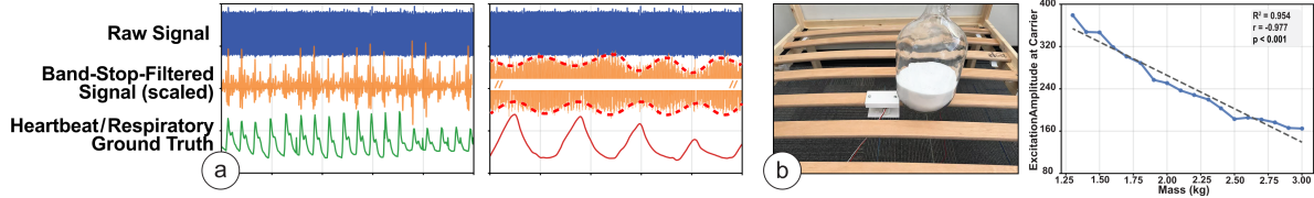
Fig. 10. Validation of frequency-domain separation and load-induced amplitude modulation. (a) Raw geophone signals and the signals after band-stop filtering for heartbeat and respiration. (b) Controlled loading experiment using a salt-filled bottle placed above the instrumented bed beam.
