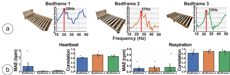
Fig. 23. Evaluation across bed frames. (a) Tested bed frames and excitation frequencies selected through impulse-response characterization. (b) Heartbeat and respiratory performance.
