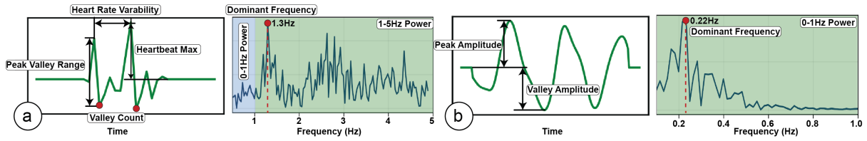
Fig. 5. Examples of (a) heartbeat-related features and (b) respiration-related features, which are extracted from separated vibration responses.
