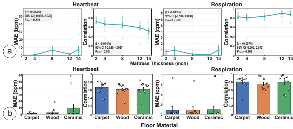
Fig. 22. Robustness across (a) mattress thicknesses and (b) floor materials.
