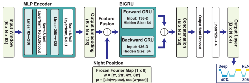
Fig. 6. The MLP–BiGRU model architecture.
