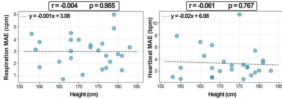
Fig. 26. Correlation between participant height and physiological signal reconstruction accuracy.
