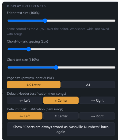
Fig. 37 — Display Preferences.
