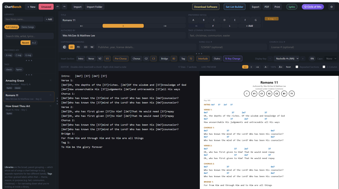
Fig. 7 — CC mode: answer two quick questions with the small letter buttons and the chart carries the exact license.
