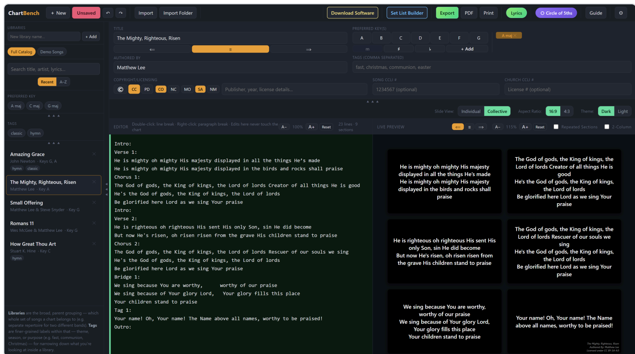
Fig. 22 — Lyrics mode, Collective view: every slide at once. One section per slide; every paragraph break starts a new slide.
