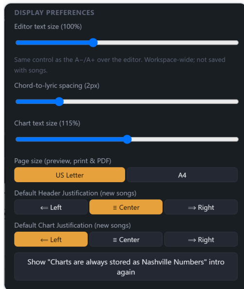
Fig. 31 — Display Preferences.
