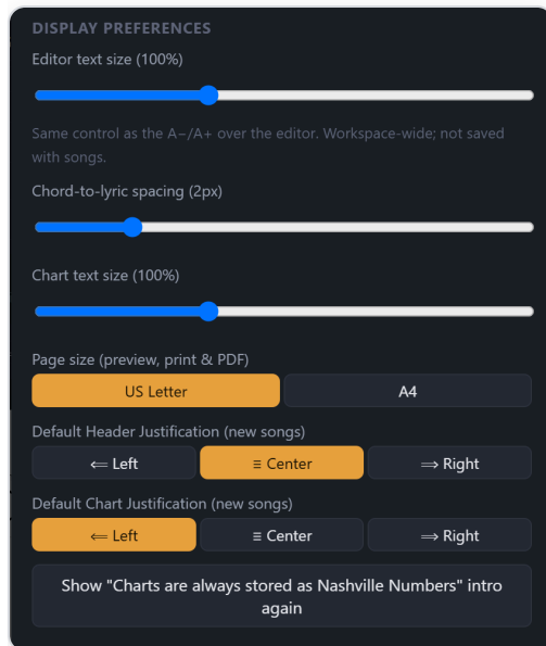
Fig. 30 — Display Preferences.
