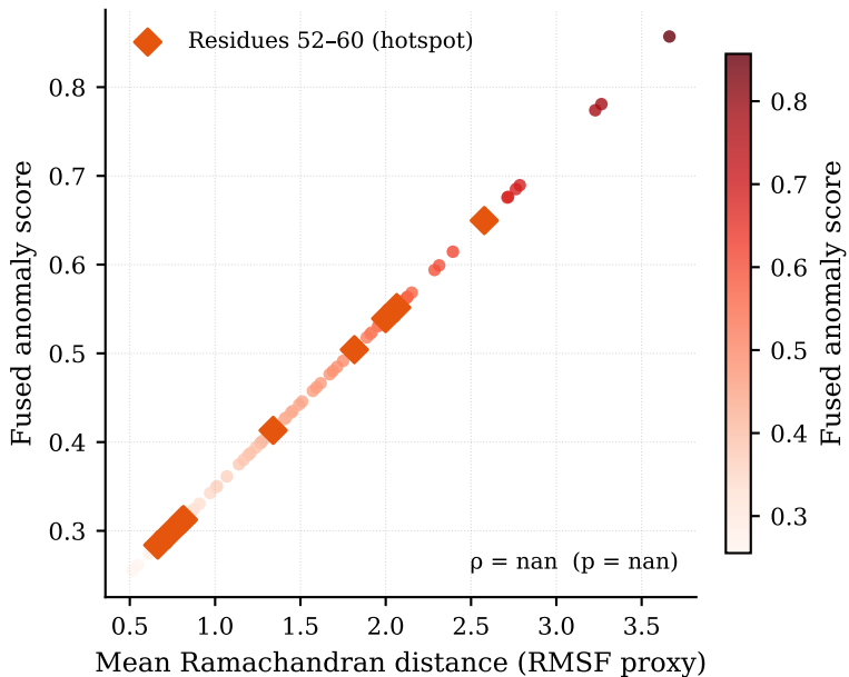
Anomaly score vs conformational flexibility (RMSF proxy)
