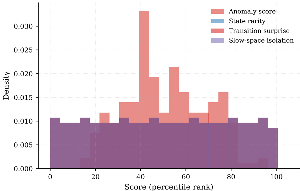
Case study: distribution of per-frame anomaly scores
