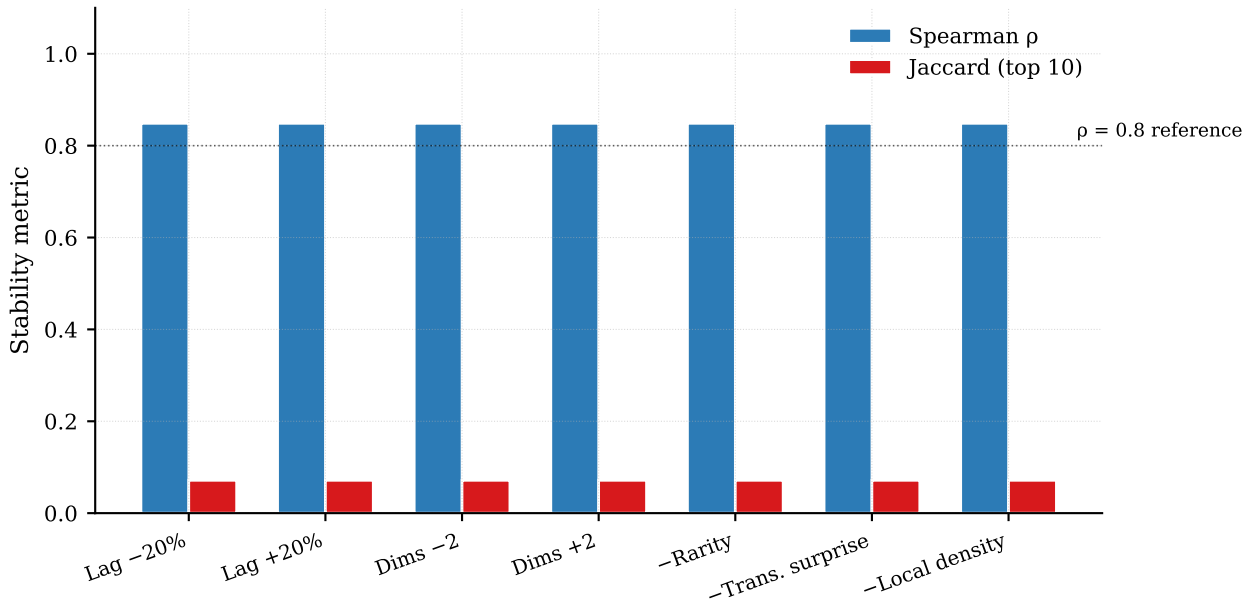
Case study: ranking stability under perturbation
