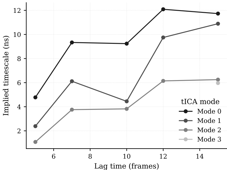
Implied timescales vs lag time
